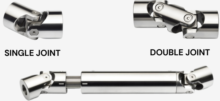
TELESCOPIC JOINT
